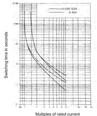
Time-current characteristic (total switch-off time at nominal voltage) Ambient temperature 23°C
